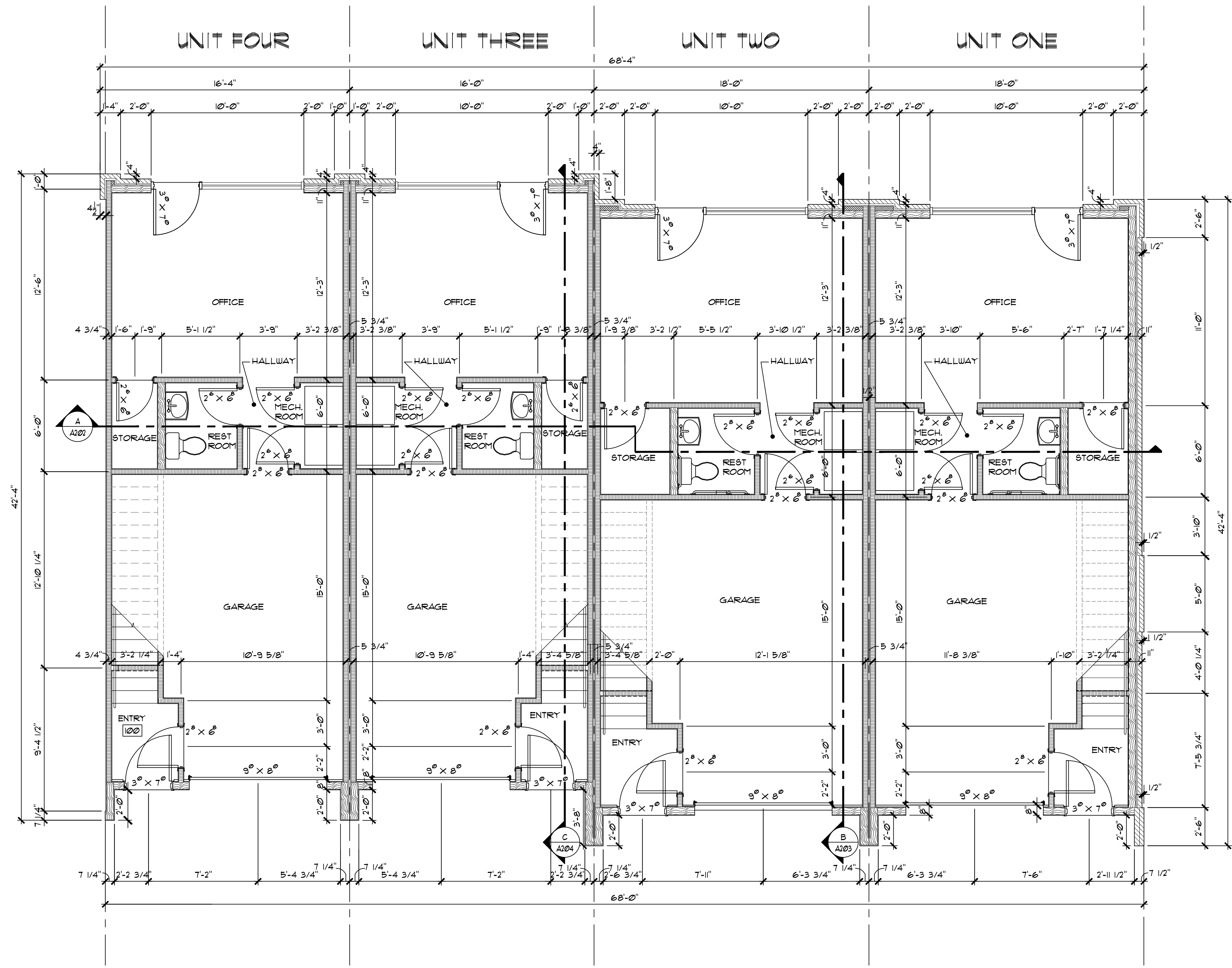
MAIN LEVEL FLOOR PLAN SCALE: 1/4" = 1'-0"
