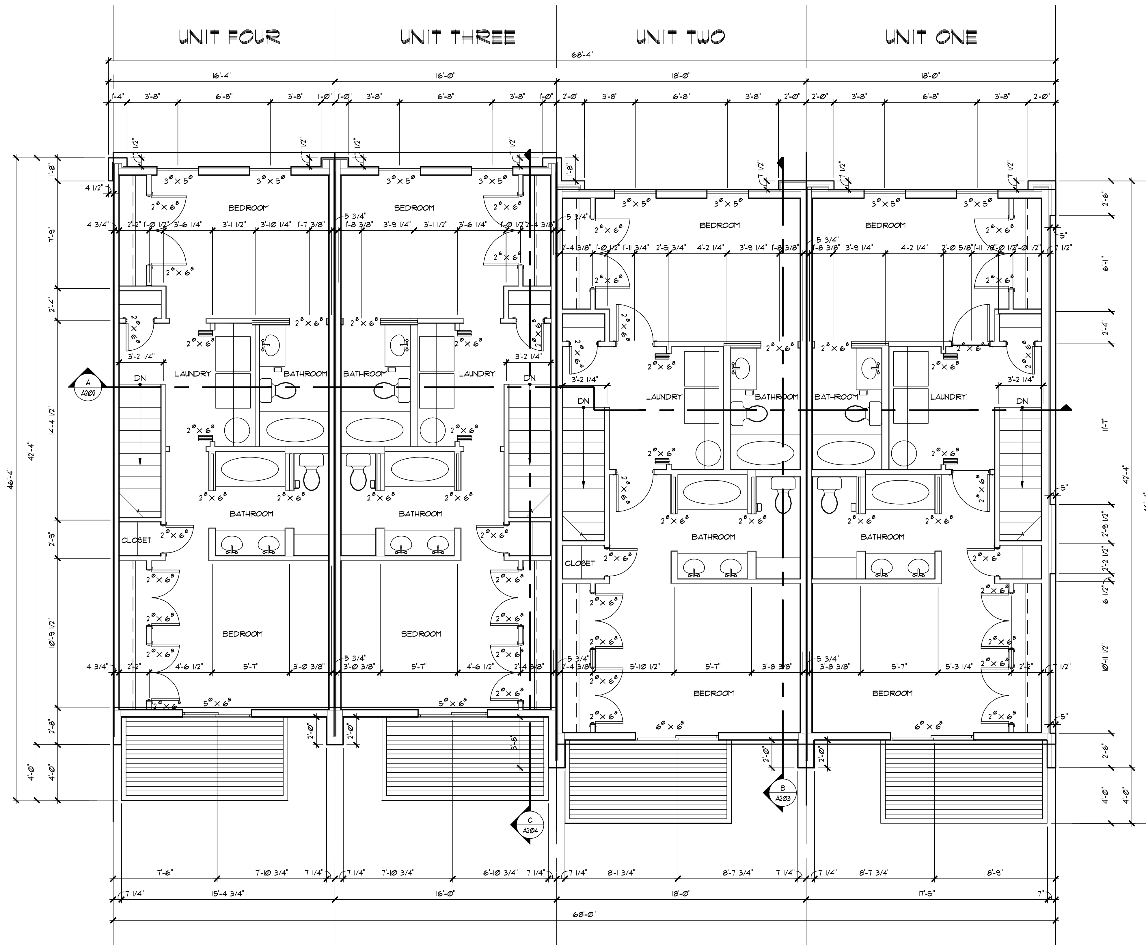
THIRD LEVEL FLOOR PLAN SCALE: 1/4" = 1'-0"
