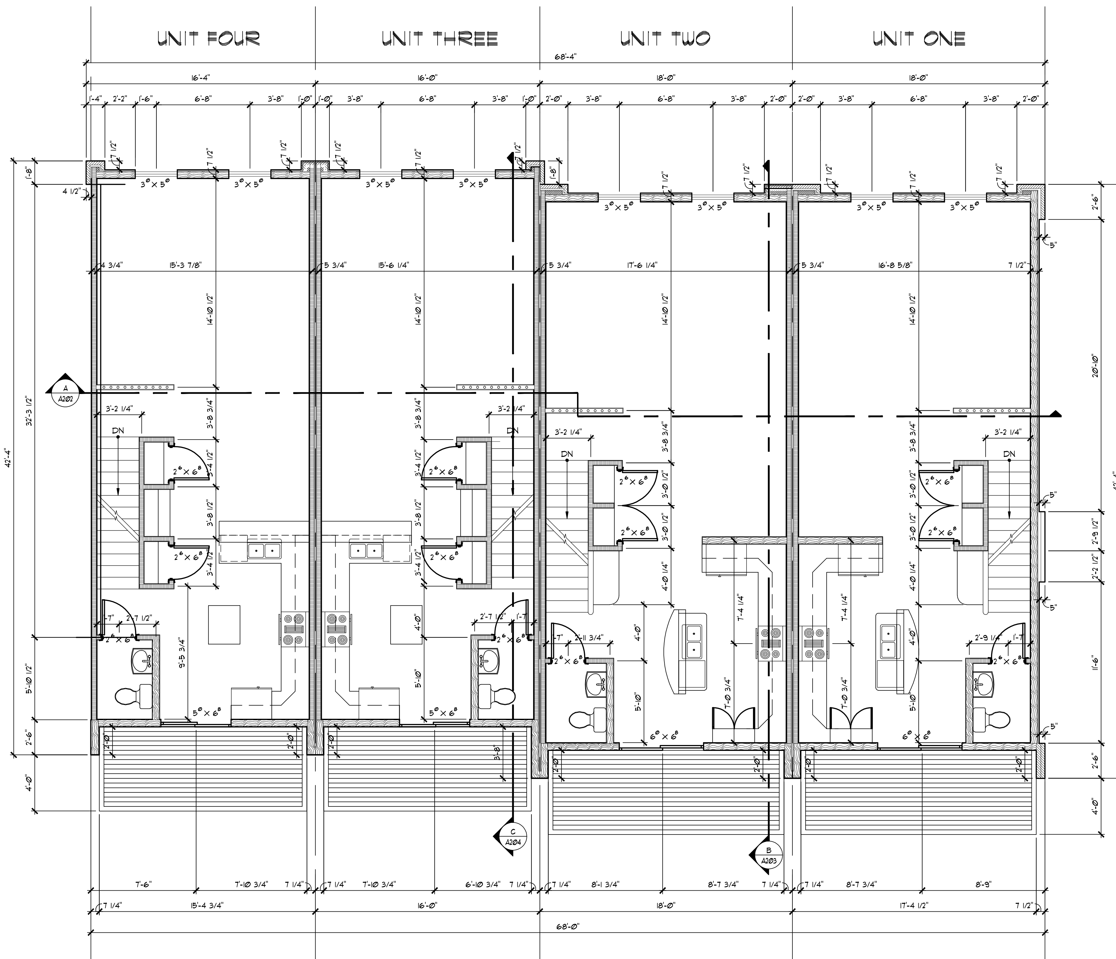
SECOND LEVEL FLOOR PLAN SCALE: 1/4" = 1'-0"
